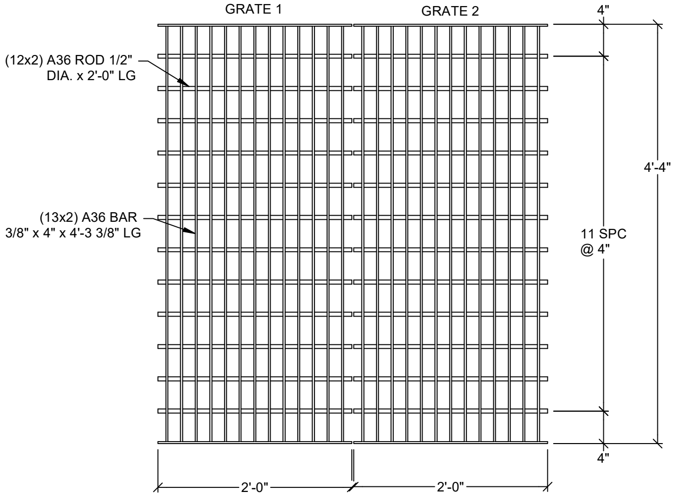
PLAN VIEW SCALE 1" = 1'-0" (A)
