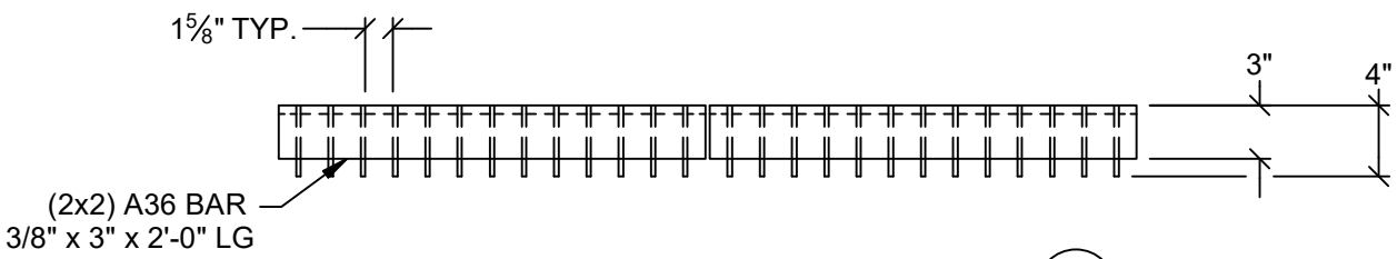
PROFILE VIEW SCALE 1" = 1'-0" (B)
