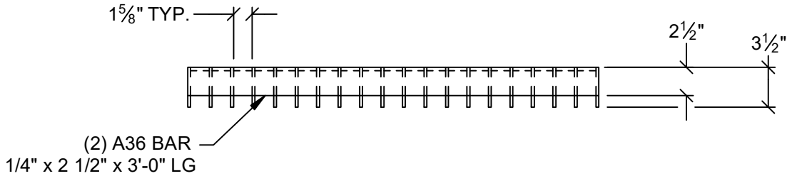
PROFILE VIEW SCALE 1" = 1'-0"
