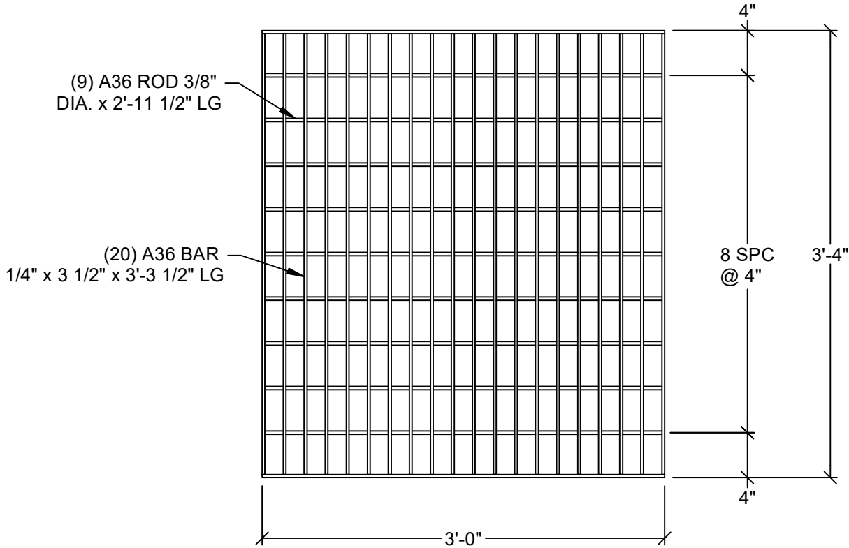
PLAN VIEW SCALE 1" = 1'-0"
