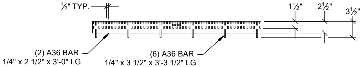
PROFILE VIEW SCALE 1" = 1'-0"
