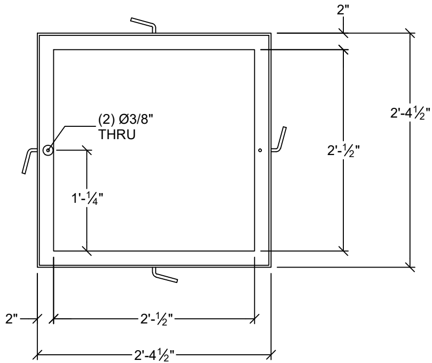
PLAN VIEW SCALE 1" = 1'-0"
