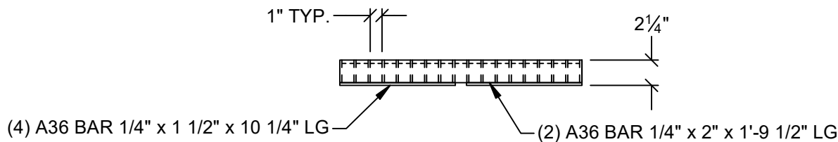
PROFILE VIEW SCALE 1" = 1'-0"
