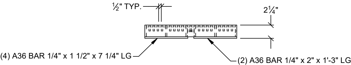
PROFILE VIEW SCALE 1 1/4" = 1'-0" B
