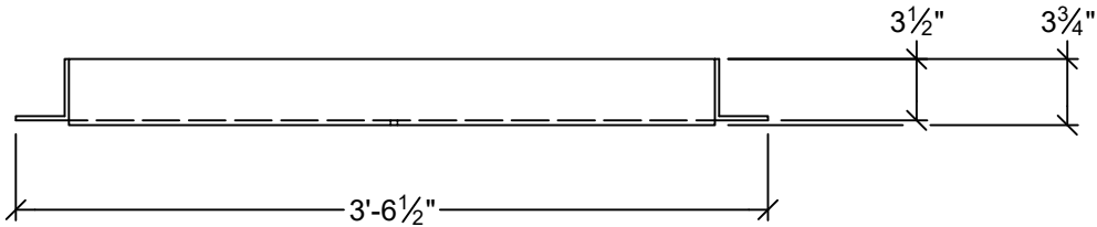
PROFILE VIEW SCALE 1" = 1'-0"
